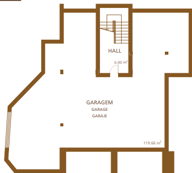
PISO -1 FLOOR -1 PLANTA -1
